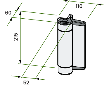
Mammoth-HD
